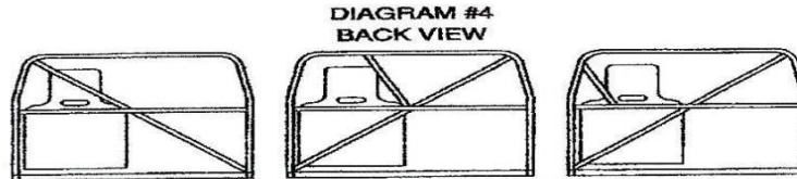
DIAGRAM #4 BACK VIEW ADDITIONAL BRACING BEHIND DRIVER'S HEAD IN MAIN HOOP REQUIRED. THESE DIAGRAMS ARE MEANT TO BE SUGGESTIONS ONLY.
