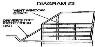
DIAGRAM #3 VENT WINDOW BRACE DRIVER'S FEET PROTECTION BAR THIS AREA TO BE .095 INCH WALL THICKNESS BY 1.66 INCH O.D. TUBING MINIMUM.
