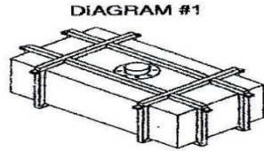
DIAGRAM #1 1 INCH STEEL SQUARE TUBING OR 2 INCH BY 1/8 INCH STEEL STRAP
