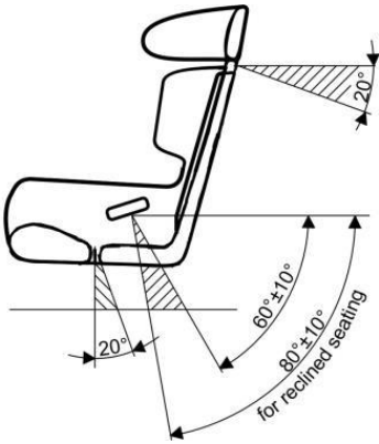
LAP BELT ANGLE
